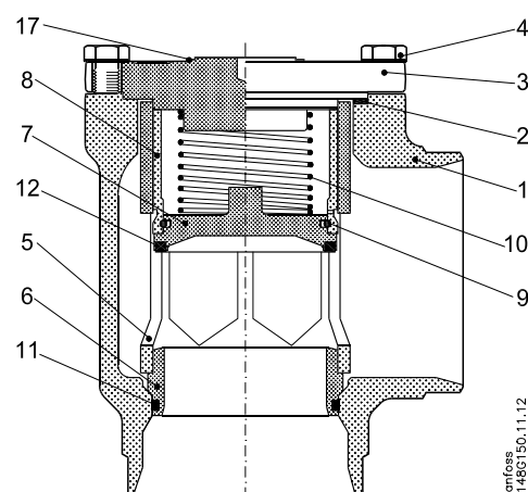
CHV-X 50 – 125
