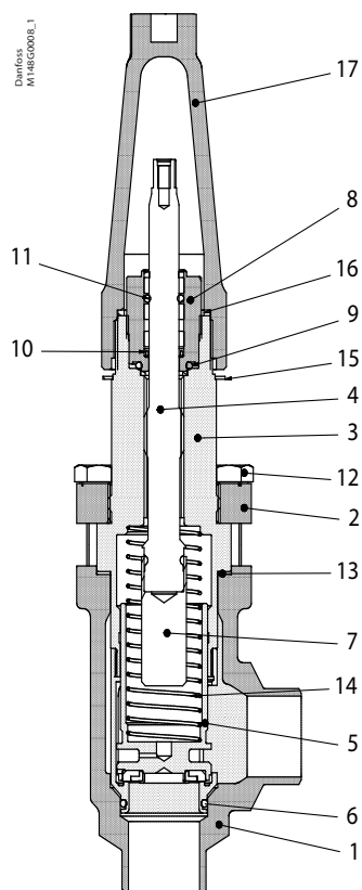
SCA-XSS 15-40
