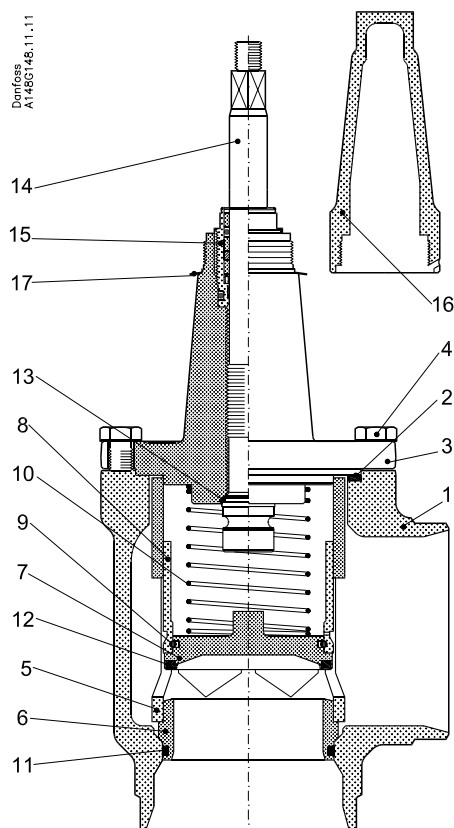
SCA-X 50 – 125
